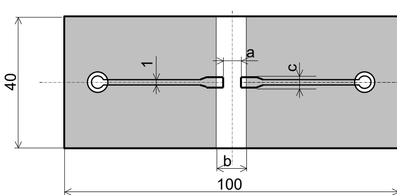
RLC50, 63 BOUND STRENGTH OF THE END FACE PLATING TEST SUBSTRATE
