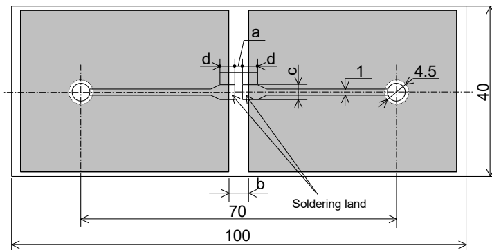
RLC10,16, 20, 32, 35 BOUND STRENGTH OF THE END FACE PLATING TEST SUBSTRATE
